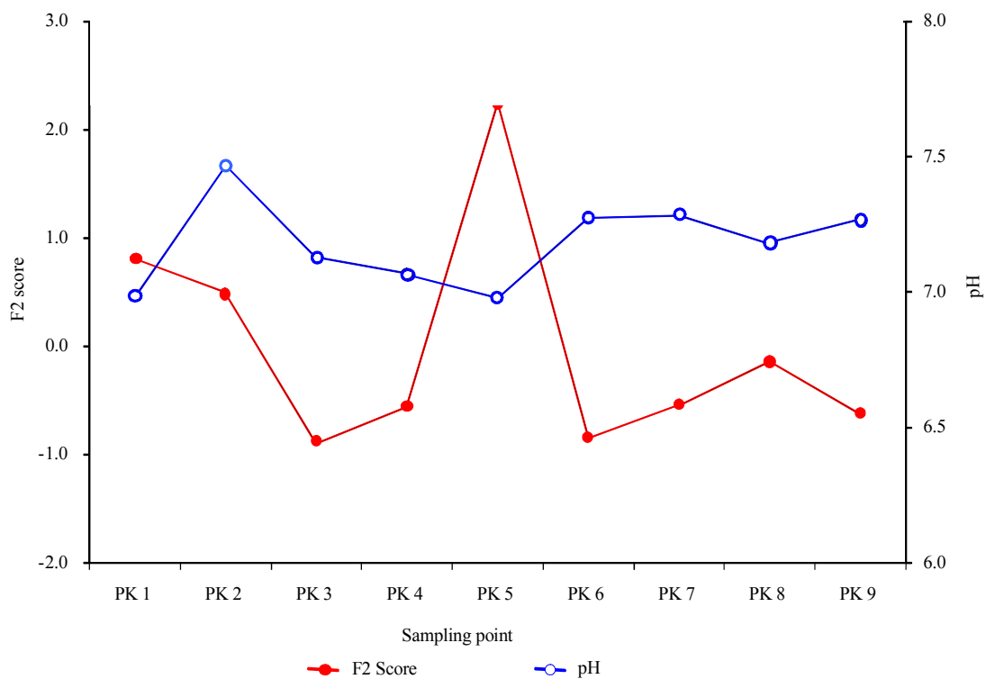
Fig. 4: The relationship between average F2 score and pH of groundwater
