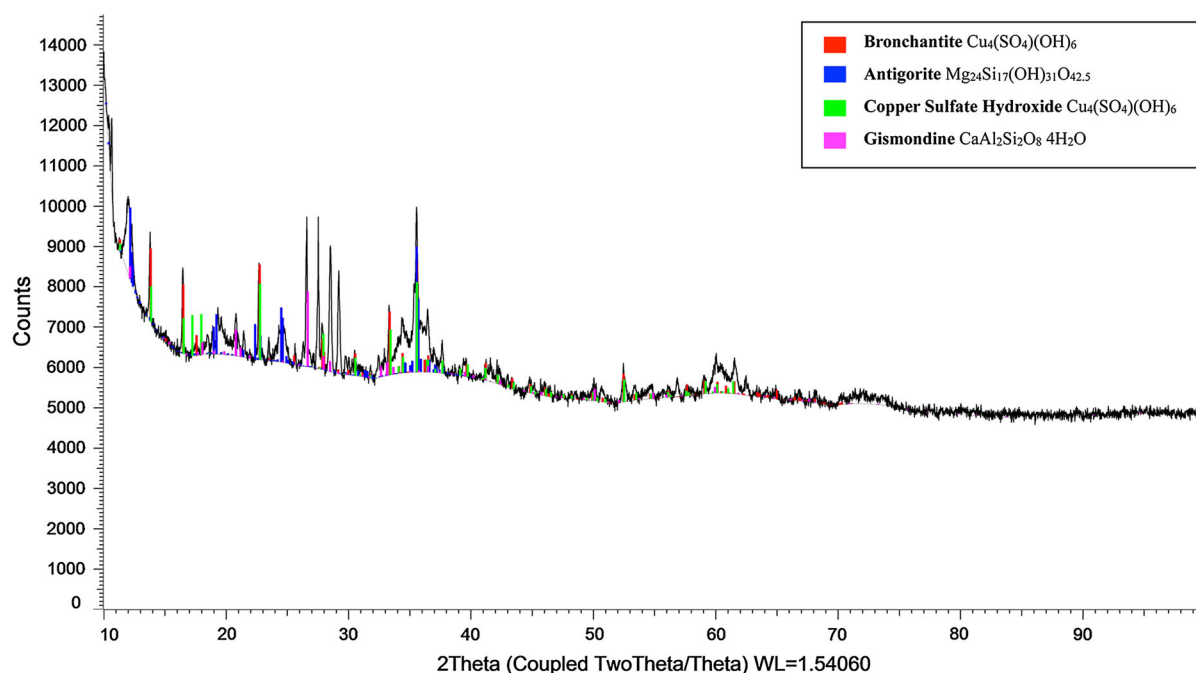
Fig. 4 XRD spectra of selected Cu precipitate sample
