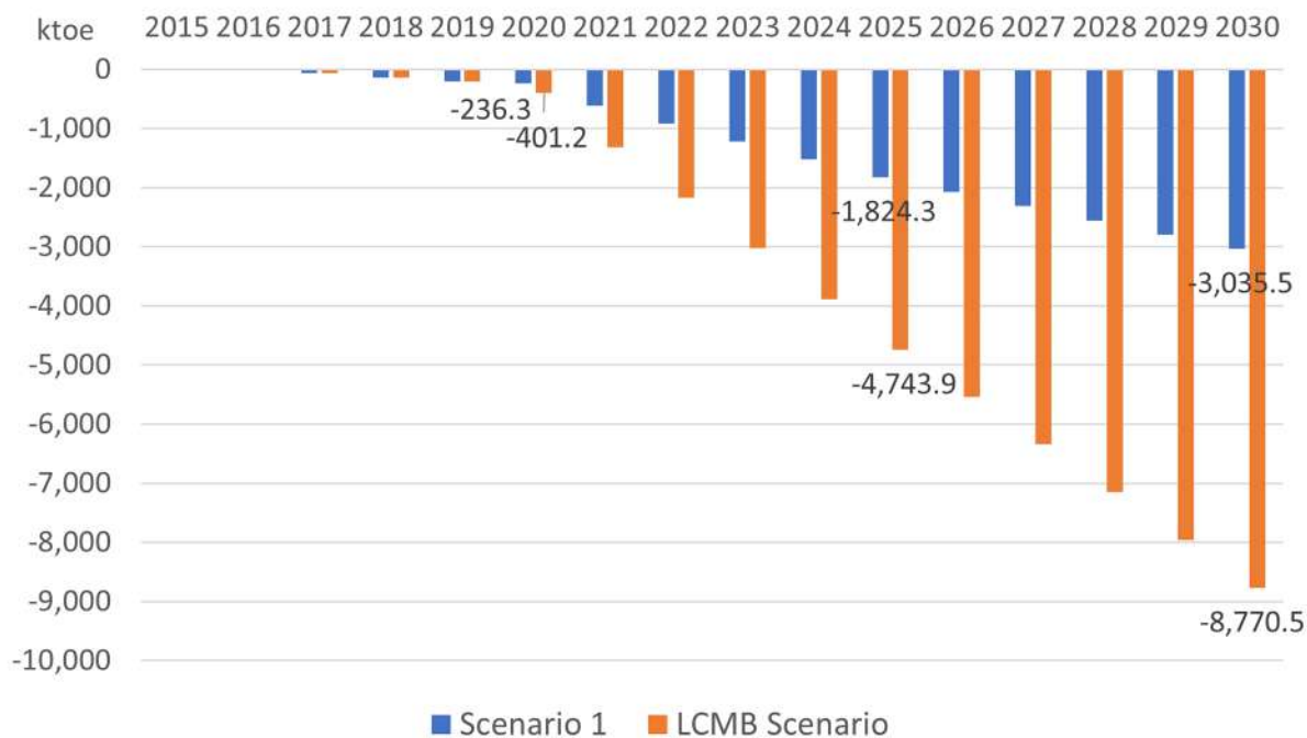
Figure 7.1: Reduction in Final Energy Consumption for Scenario 1 and LCMB Scenario (Source: LEAP Model Output)
