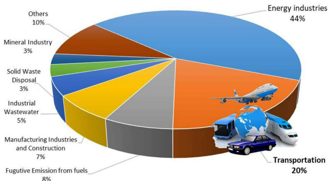
Figure 1.2: Greenhouse Gas (GHG) emission by sector, 2014
