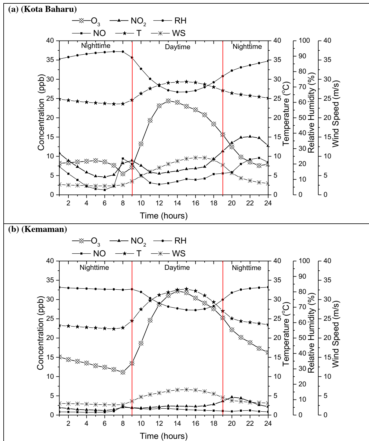
Figure 2. Diurnal variation of ozone, nitric oxide, nitrogen dioxide, temperature, relative humidity and wind speed at (a) Kota Baharu, Kelantan and (b) Kemaman, Terengganu.
